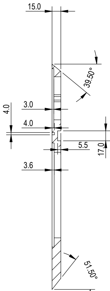
SECTION H-H SCALE 1 : 4
